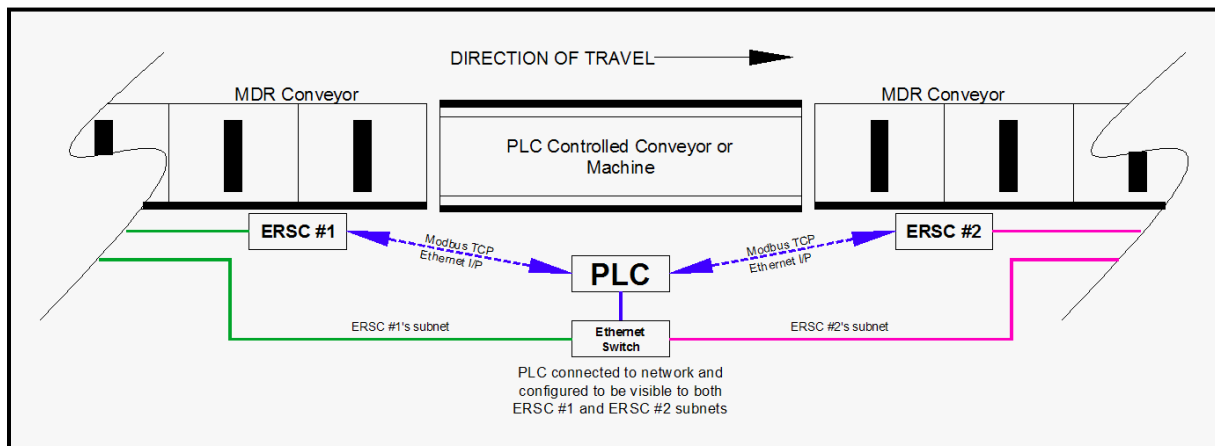
FIGURE 12 - PLC CONVEYLINX BRIDGE
