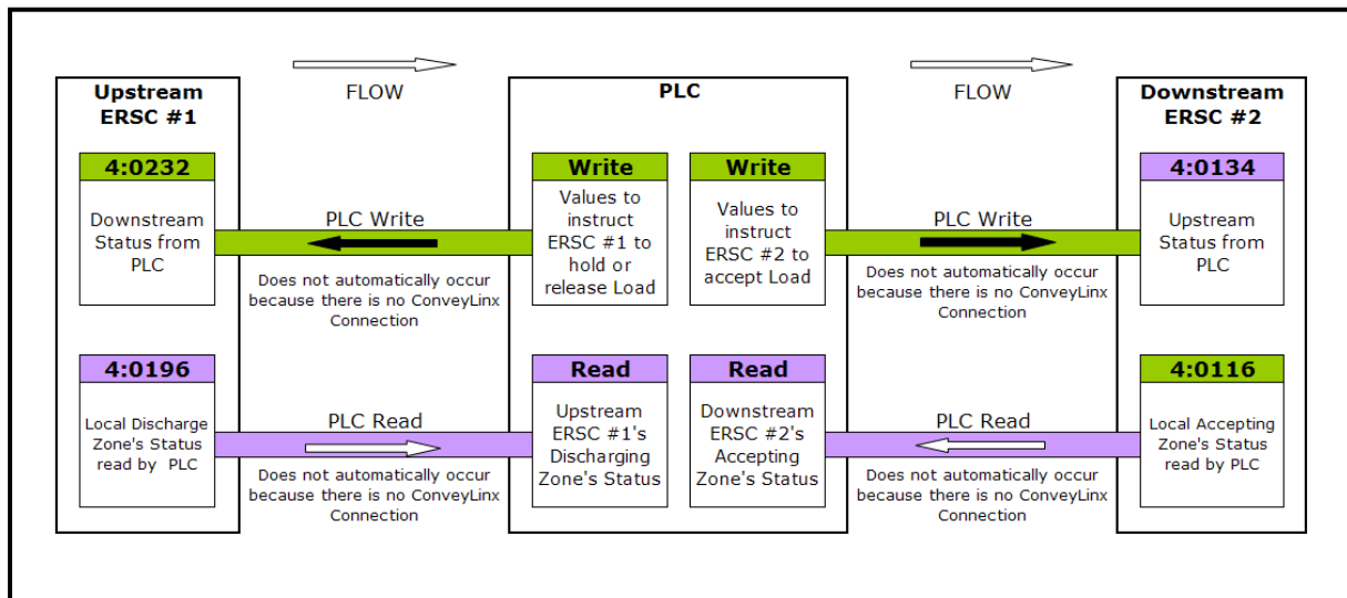
FIGURE 13 – DATA FLOW CHART FOR PLC CONVEYLINX BRIDGE EXAMPLE
